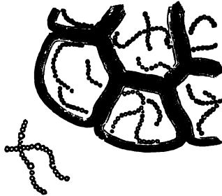
FIG. 56.— LEUCONOSTOC MESENTEROIDES ; COCCI-CHAINS WITH ARTHROSPORES (after Van Tieghem and Cienkowski).
